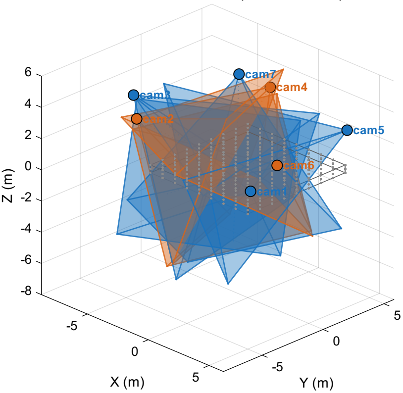
GA-best — 7 cams (Cost: 0.0185)
